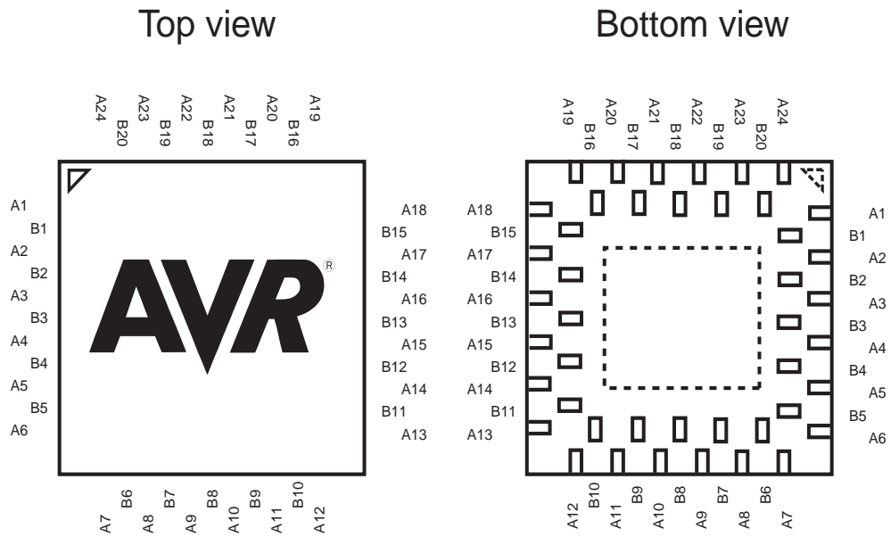
Figure 1-2. DRQFN - pinout.
